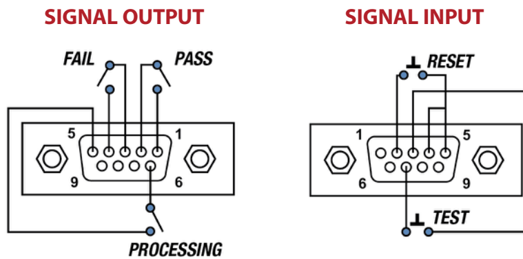
Figure 1 Pin Configurations for Remote I/O
